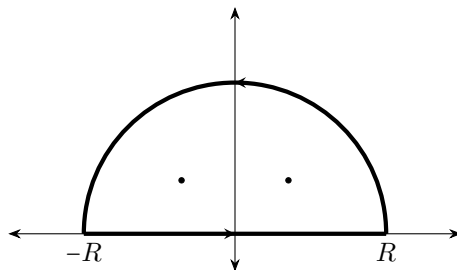
Figure 9: Contour in the upper half-plane, with the two points denoting the two simple poles of f(z) in the upper half-plane.
