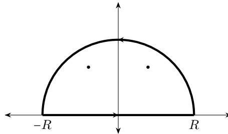
Figure 7: Contour in the upper half-plane, with the two points denoting the two simple poles of f(z) in the upper half-plane.
